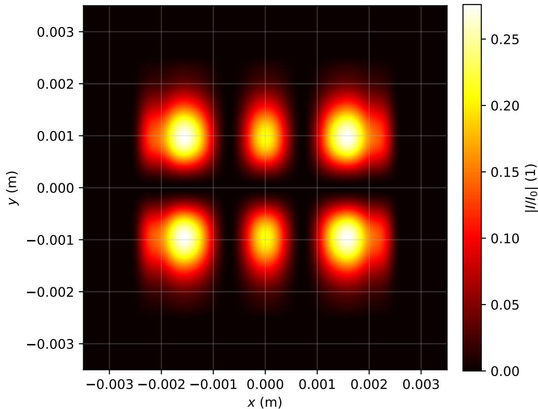
Intensity profile I(x, y, z = 3.423)/I_0 , P_{in}=0.5P_{cr} , artificial time
